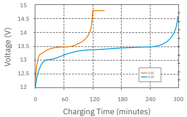
Charging Characteristics at 0.2C and 0.5C Charging (25°C Ambient Temperature)
